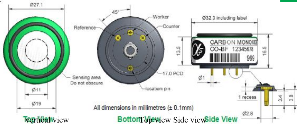
Figure 1 schematic diagram of CO-BF
