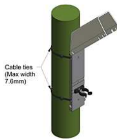
Post mounting Use 2 off suitable cable ties threaded through holes in backplate as shown
