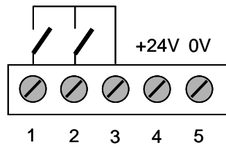
Fig. 2: Connection layout for AQ-CONTROL. Relay contact terminal 2: pulse at [\text{CO}_2] > 1,500 ppm; relay contact terminal 1: pulse at [\text{CO}_2] < 1,400 ppm
