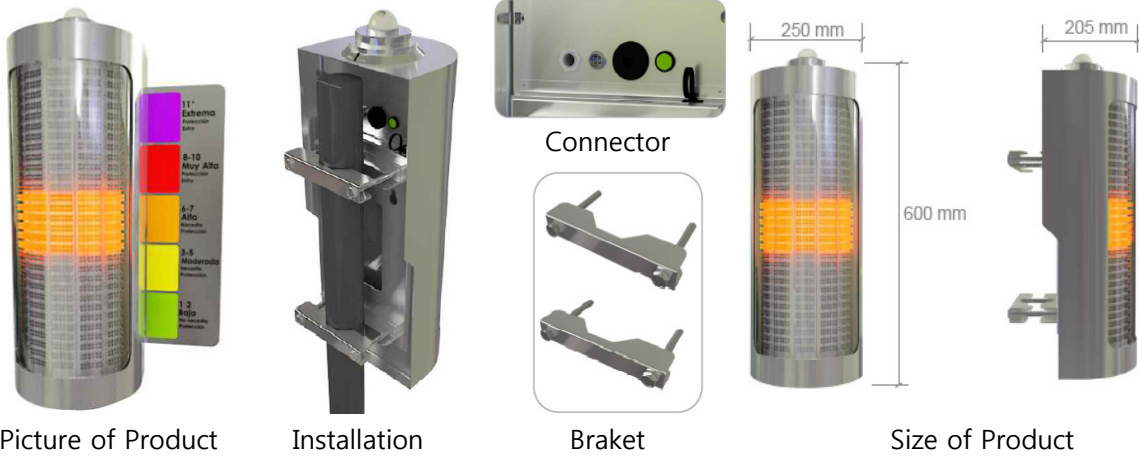
Fig1. Physical Dimentions
